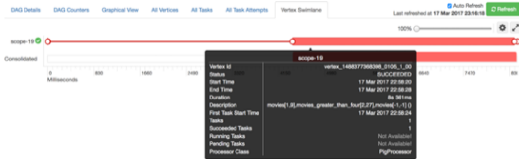
Figure 11.13. Tez View Vertex Swimlane Tab
