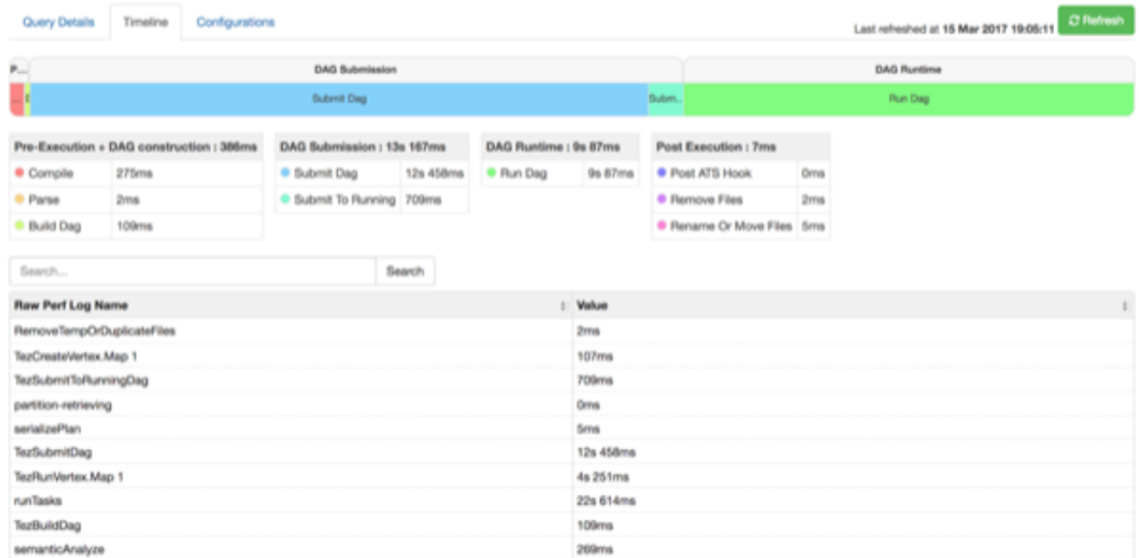
Figure 11.5. Total Timeline and Log Details of a Submitted Query
