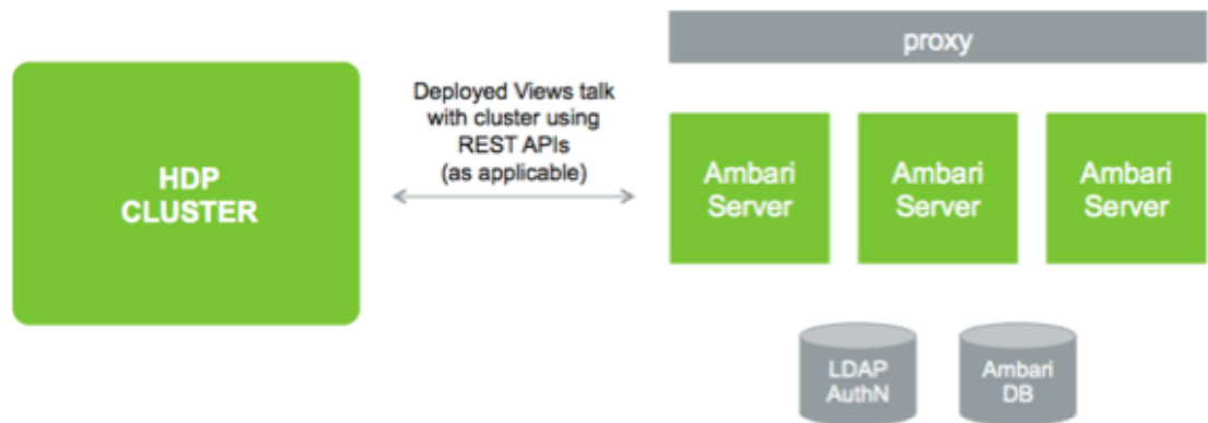
Figure 2.1. Configuring Views with your HDP Cluster
