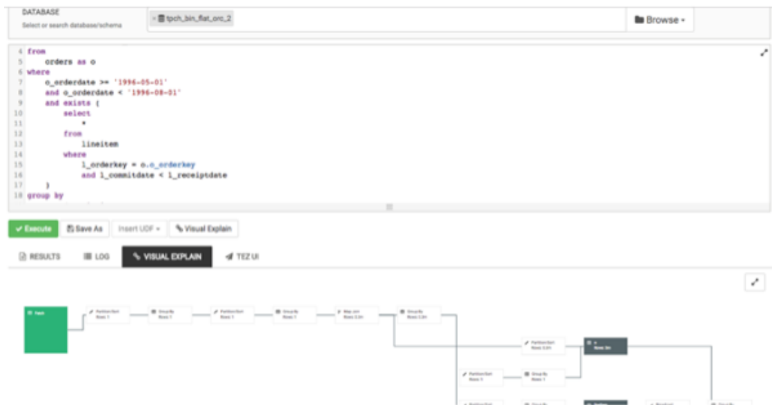
Figure 6.5. SQL in Query Editor with Resulting Visual Explain Plan
