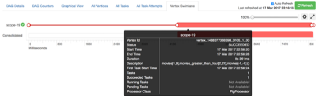
Figure 11.13. Tez View Vertex Swimlane Tab
