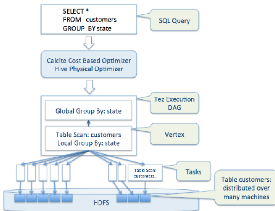
Figure 11.2. SQL Query Execution in Hive
