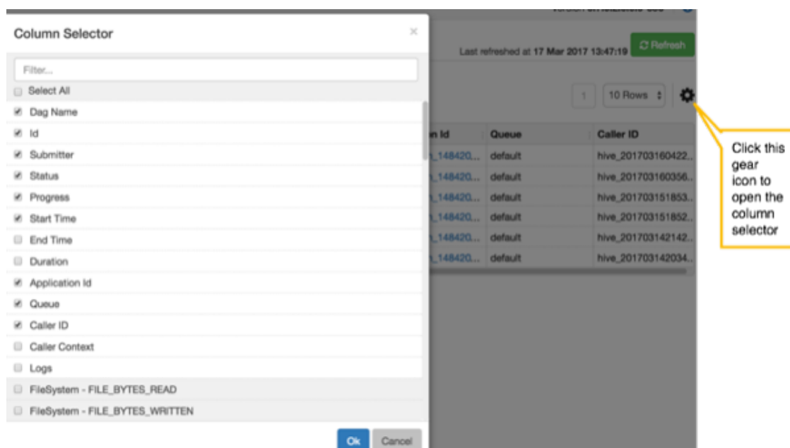
Figure 11.8. Tez View Column Selector Dialog Box
