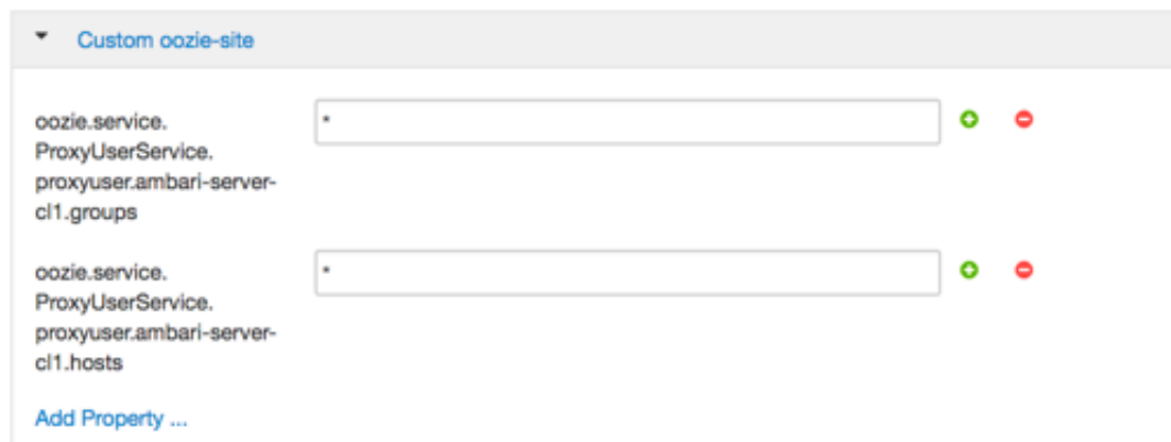
Figure 2.17. wfm-oozie-proxy-user.png
