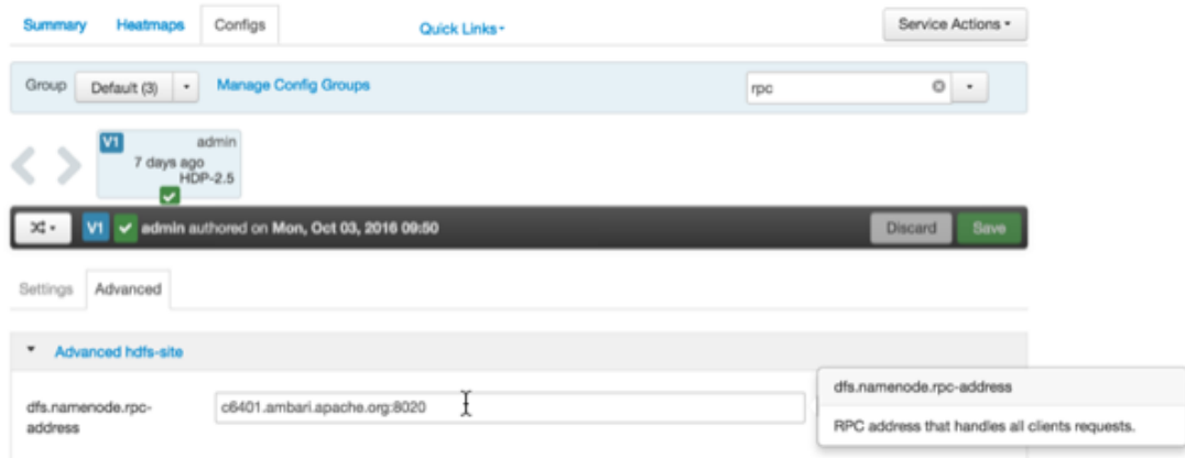
Figure 2.10. Using the Filter to Search Advanced hdfs-site Settings
