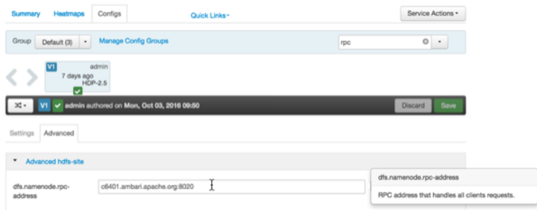
Figure 2.5. Using the Filter to Search Advanced hdfs-site Settings
