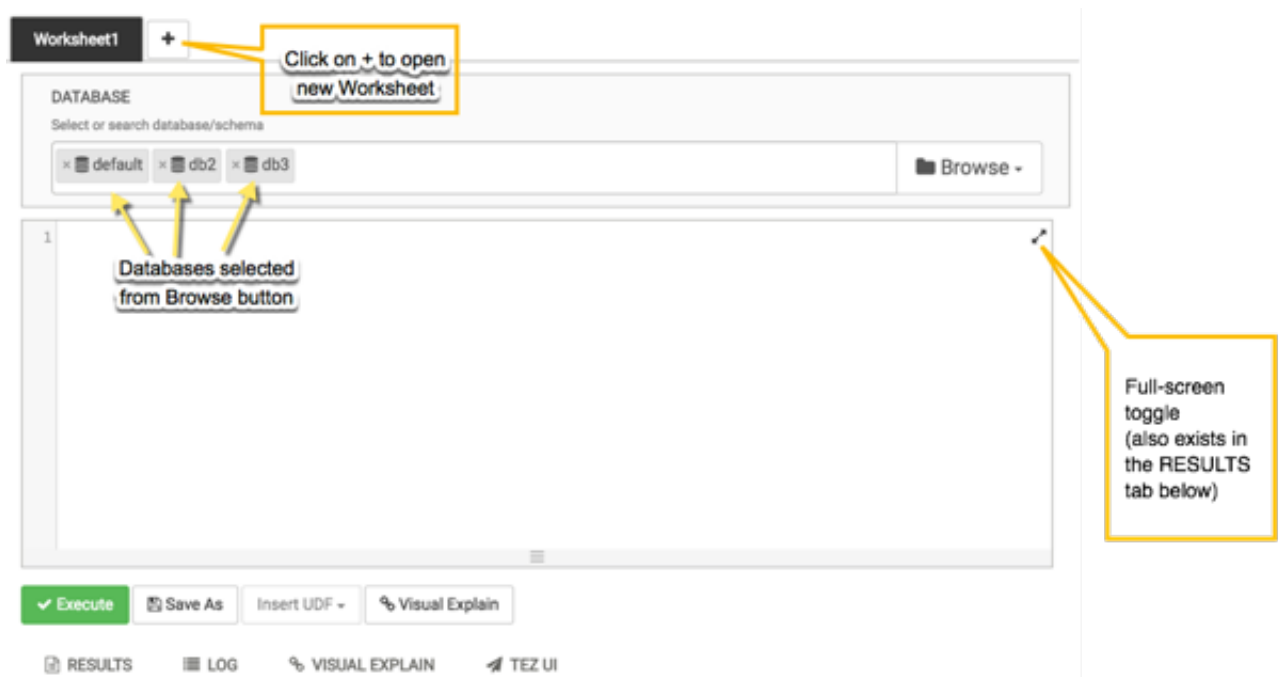
Figure 6.3. Query Editor
