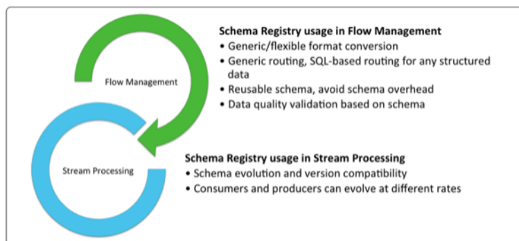
Figure 4.1. Schema Registry Usage in Flow Management
