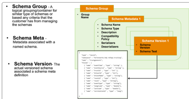
Figure 4.2. Schema entities
