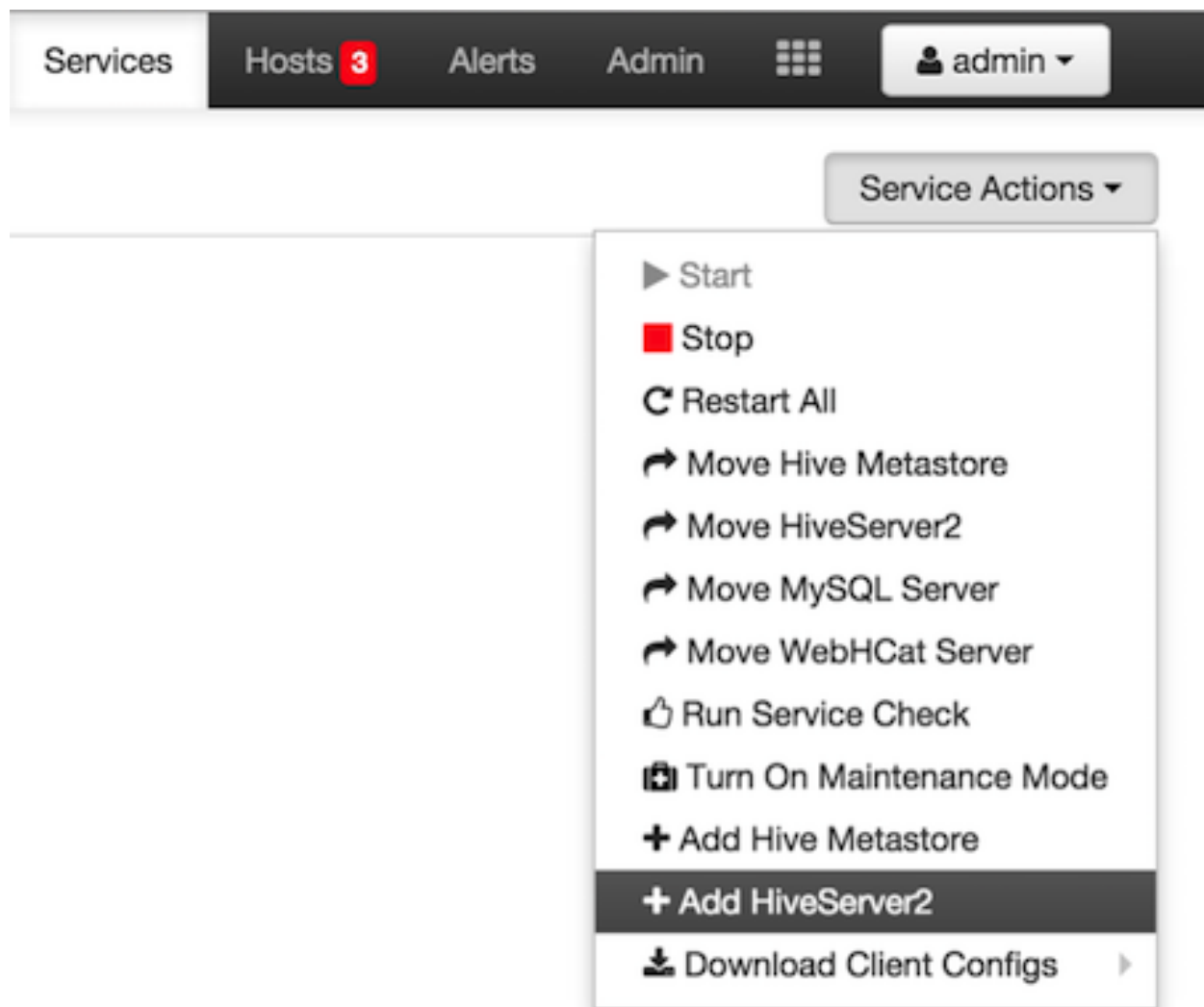
Figure 2.3. Add HiveServer2 with Ambari
