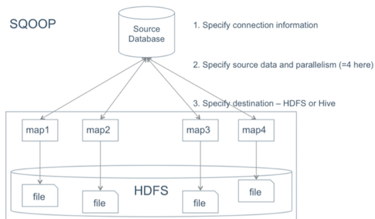
Figure 1.2. Using Sqoop to Move Data into Hive
