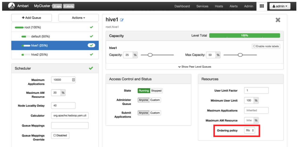
Figure 3.11. Ordering Policy Setting in Ambari
