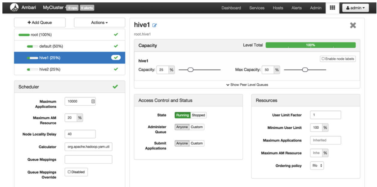
Figure 3.8. Ambari Capacity Scheduler View
