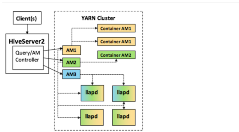
Figure 2.10. LLAP on Your Cluster
