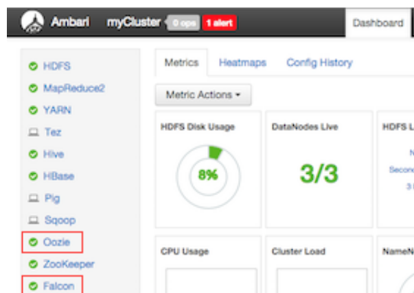
Figure 7.1. Ambari Dashboard Falcon and Oozie Service Indicators
