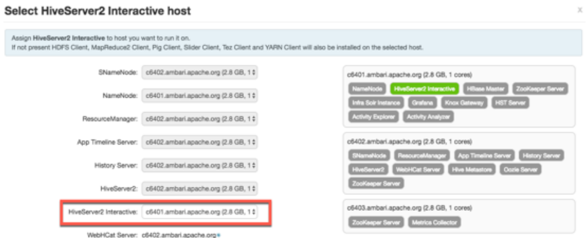
Figure 1.3. Select HiveServer2 Interactive Host Window
