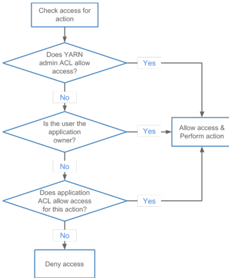
Figure 5: Application ACL Evaluation Flow
