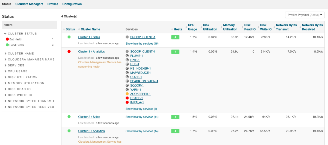
Figure 1: Multi Cloudera Manager Status Dashboard
