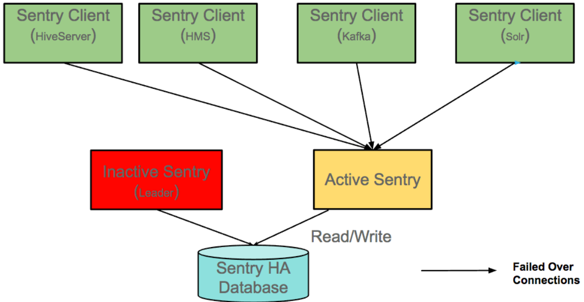
Figure 3: Sentry High Availability Architecture with Failover
