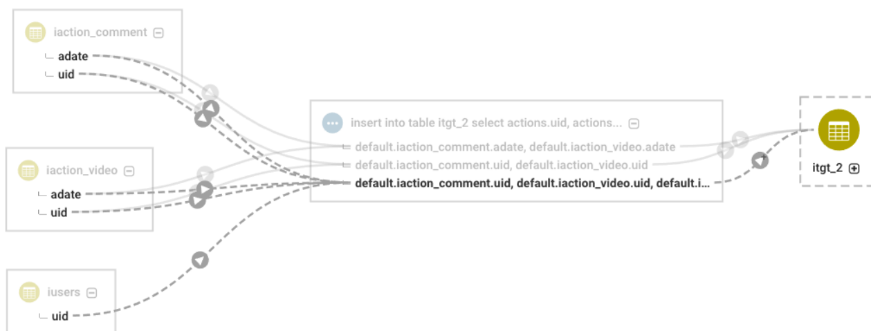
Figure 3: Lineage Showing Control Flow Relations at the Column Level
