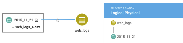
Figure 4: Logical Physical Relationship between HDFS File and Hive Table
